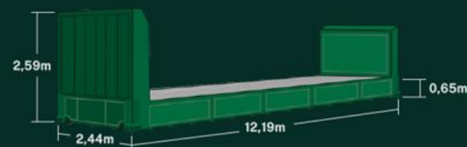
Flat Rack 40'
